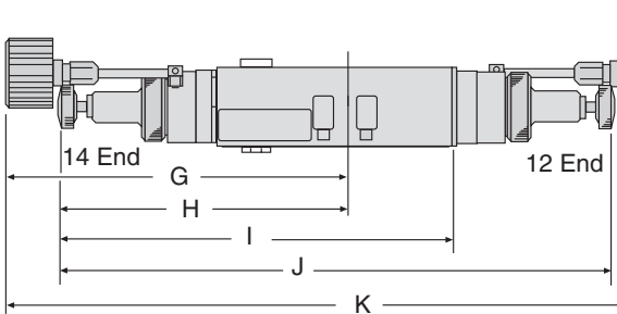
Double Interposed Regulator (top view)
